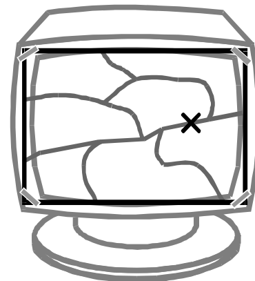
Figure II.27. Heads-up digitizing
